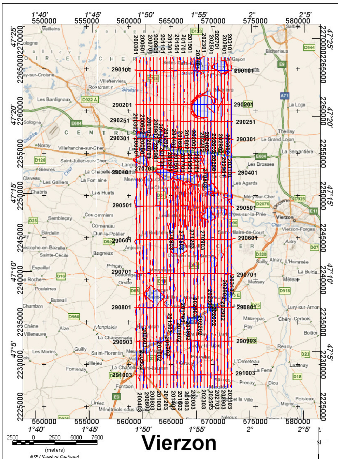
Figure 18 Red lines represent actually flown lines in respect to planned flight lines (blue). Coordinate French Lambert II (Datum: NTF Paris).
