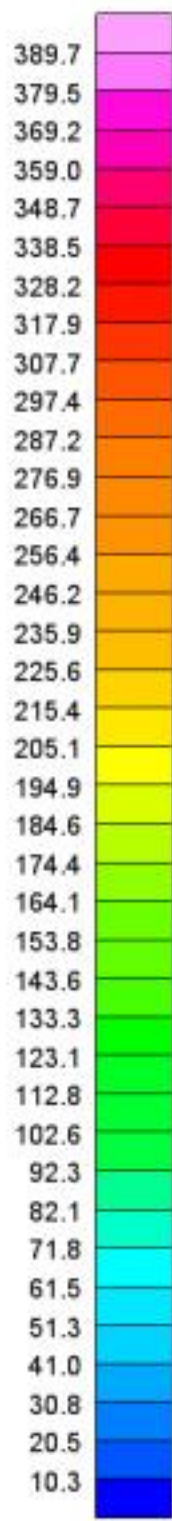
Potassium (%K)
