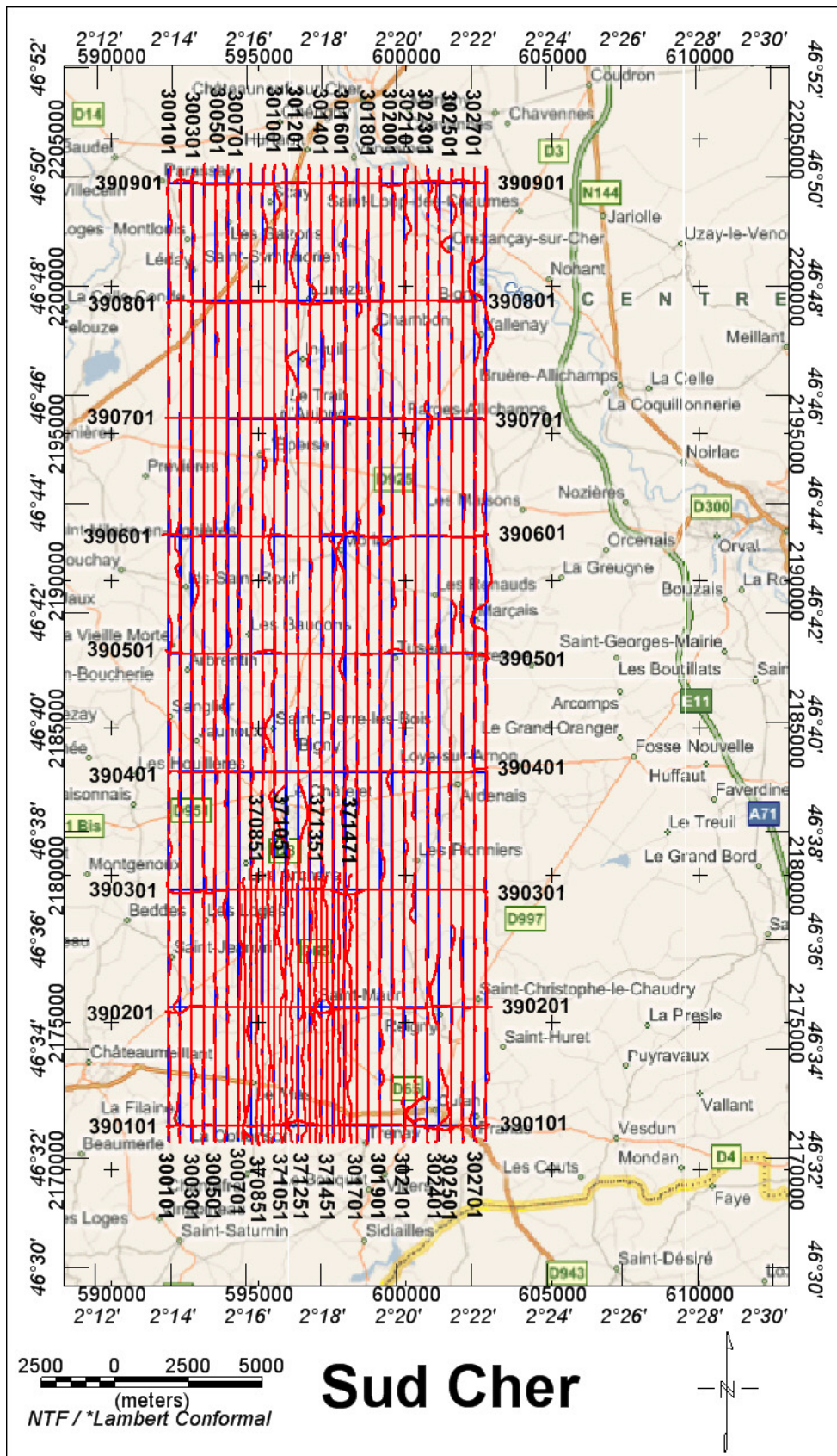
Figure 19. Red lines represent actually flown lines in respect to planned flight lines (blue). Coordinate French Lambert II (Datum: NTF Paris).
